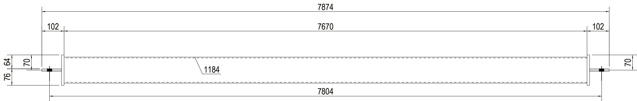
FRONT VIEW
